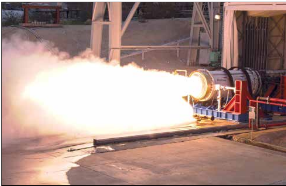
Aerojet Rocketdyne's successful qualification test of eSR-19, with the Air Force Research Laboratory at an AFRL test facility at Edwards Air Force Base, California. Photo courtesy of Aerojet Rocketdyne
