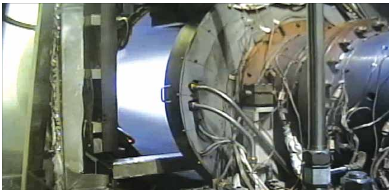
Aerojet Rocketdyne completes a successful series of hot-fire tests of an advanced air-breathing hypersonic engine under the USAF's MSCC program. Some of the camera titling has been removed for a clearer image. Photo: Aerojet Rocketdyne
