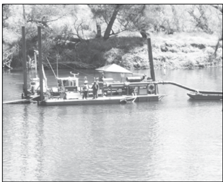
Hydraulic Dredge at Yuba City.
